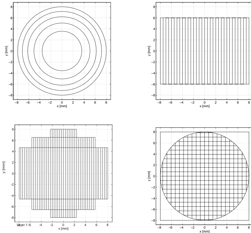
Fig. 1. Array types: Annular array, rectangular array, 1.5D array, and 2D array
