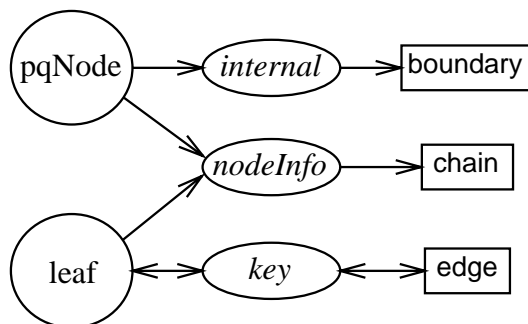
Figure 4.16: The data structure of pqtrees
