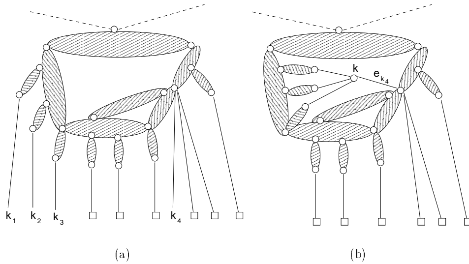
Figure 6.7: Example of embeddable edge not discovered by the PQ -tree. Shaded areas are embedded biconnected components.
